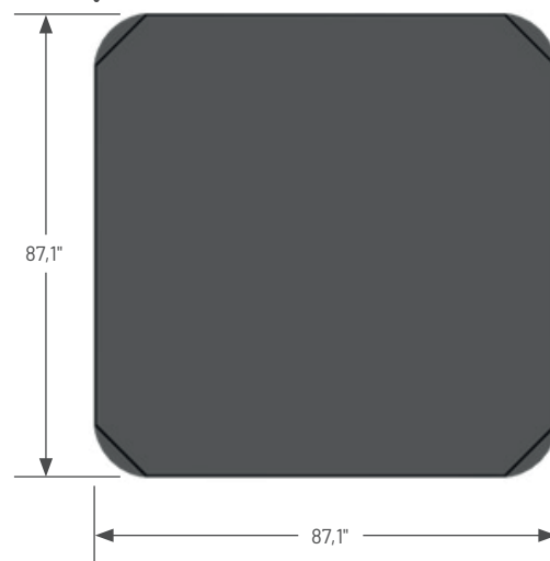
Bottom View Tolerance \pm 0.5" (1.27cm)
